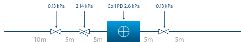
Figure 3.1.4 DN150 pipe with 20 L/s flow with a 70 [Pa/m] pipe gradient
