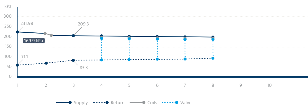
Figure 3.5.2.4 Pressure gradient for a variable primary controlled by a distributed pumpings sensor at the decoupler - 50% flow
