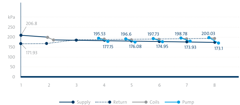
Figure 3.5.1.3 Pressure gradient for a distributed pumping system design at 50%
